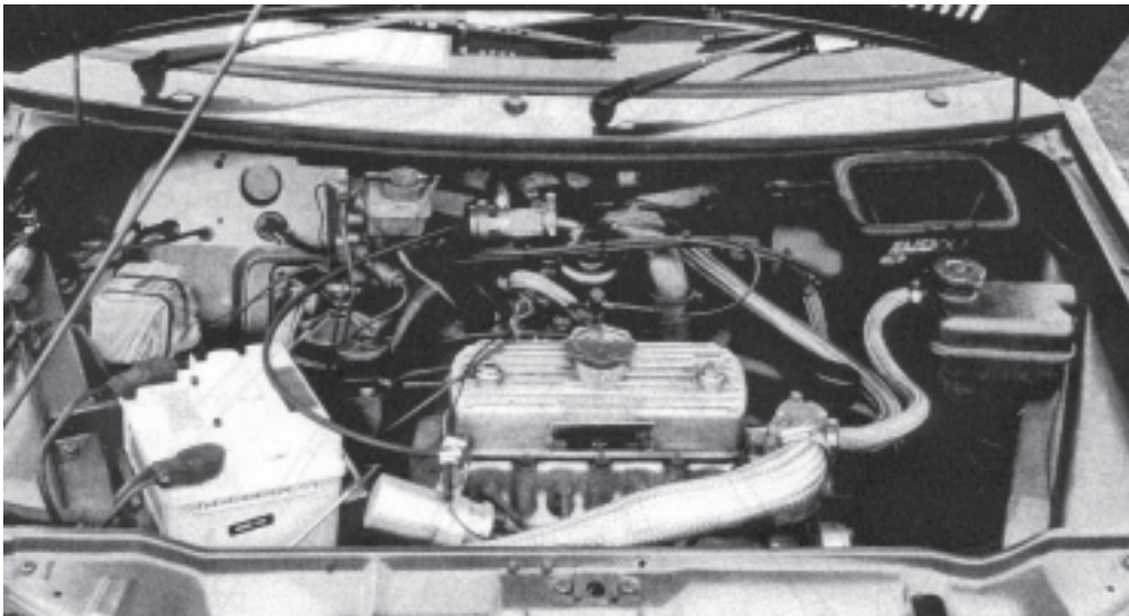
Turbo charged MG Metro engine, using the 1275cc 'A' series.
