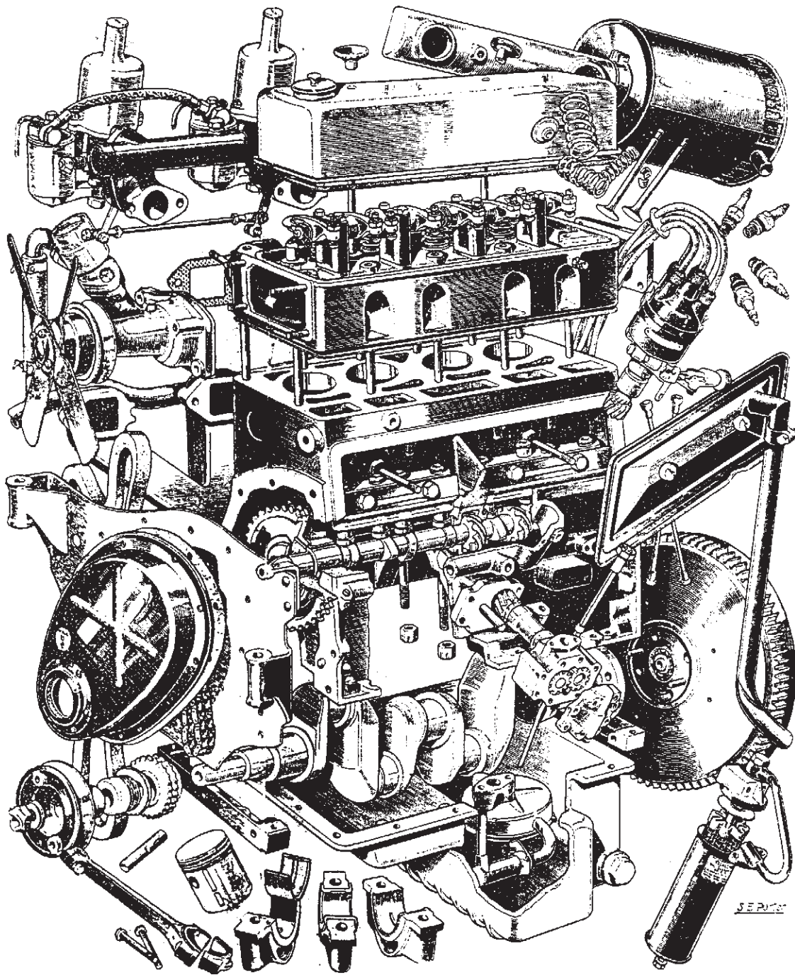
An exploded view of the MG TA Midget version of the Morris 10/4 series 3, and Wolseley 10/40 ohv engine of 1292cc. A long stroke with a narrow bore unit common of the inter-war years when the RAC formulae for road taxation was used. It was a development of the earlier Morris 10/4 s2 side valve engine. Unusually in the MG installation it has triple valve springs per valve.
