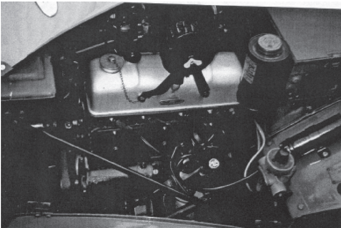
A similar engine, fitted to a MG YA, with a separate oil filter.
