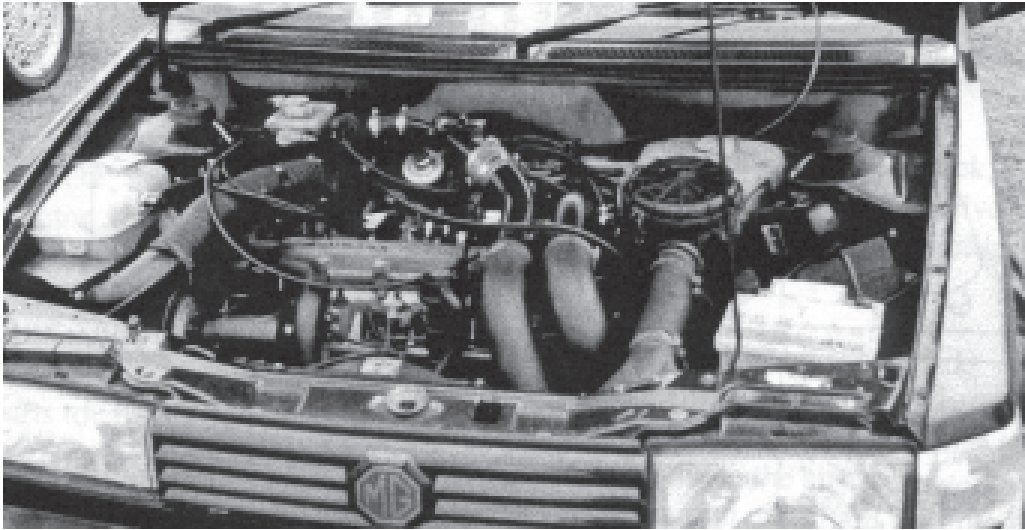
Turbo charged MG Maestro engine bay , using th e'O' series.
