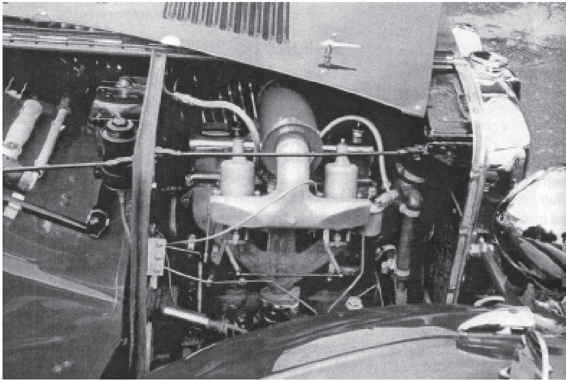
The MG VA 1292cc engine, a close relative to the Morris Twelve/4, and the Wolseley 12/40. The MG uses twin semi-downdraft carburetors.
