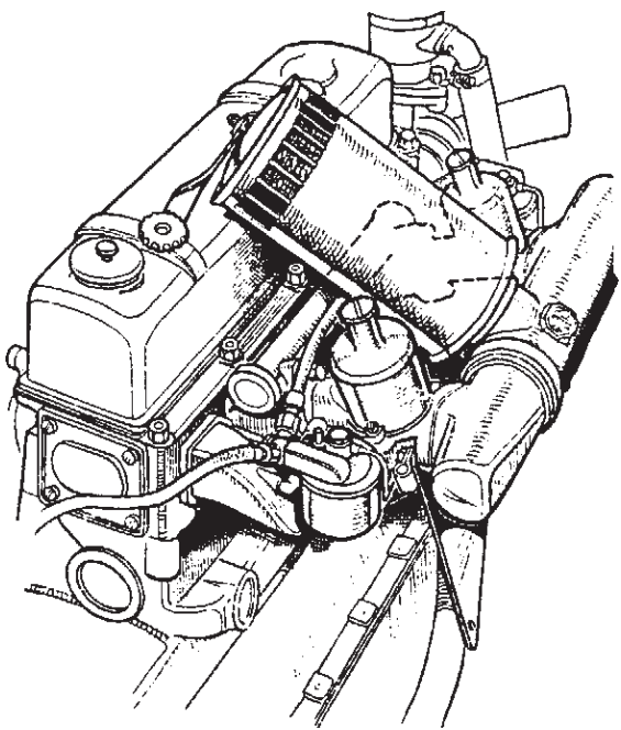
Twin carburettors are fitted to the new MG TB Midget engine.
