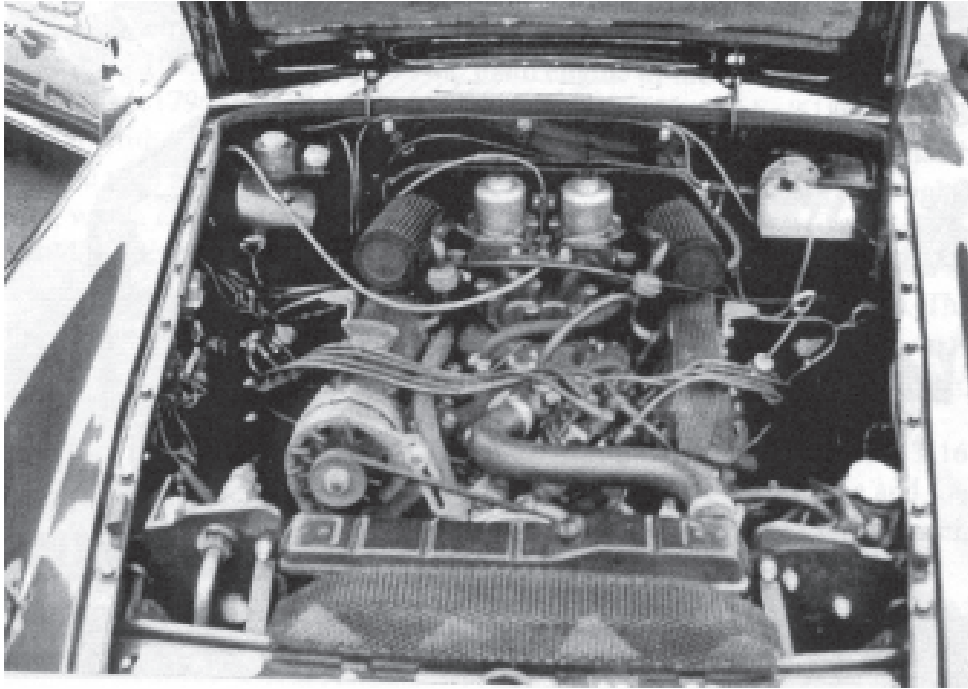
The MG factory version of the Rover V8 in an MGB, with aftermarket filters.
