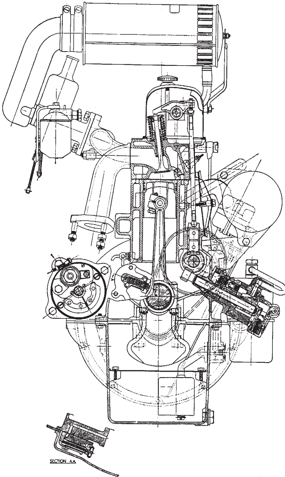
End view of the XPAG/SC 1250cc single carburetter Y saloon engine of 1947.
