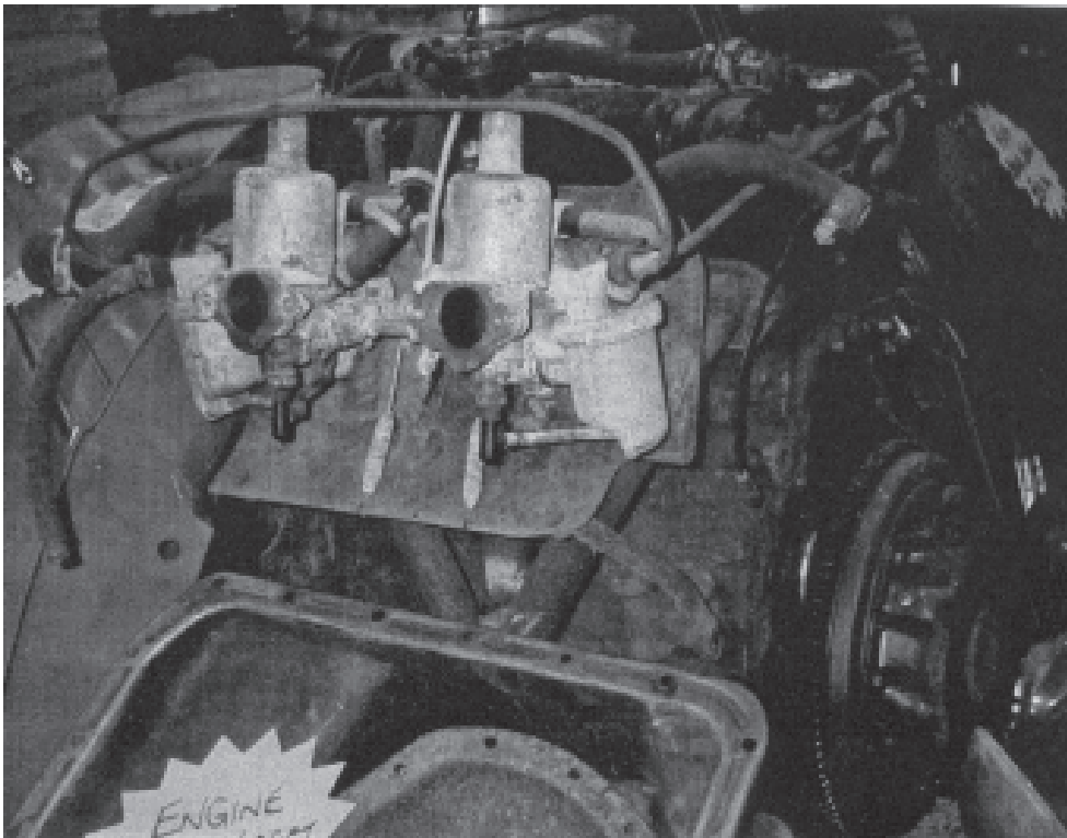
A MG Midget 1275cc 'A' series on sale at an autojumble. Take care at such locations, the engine number prefix needs checking you want the right unit.
