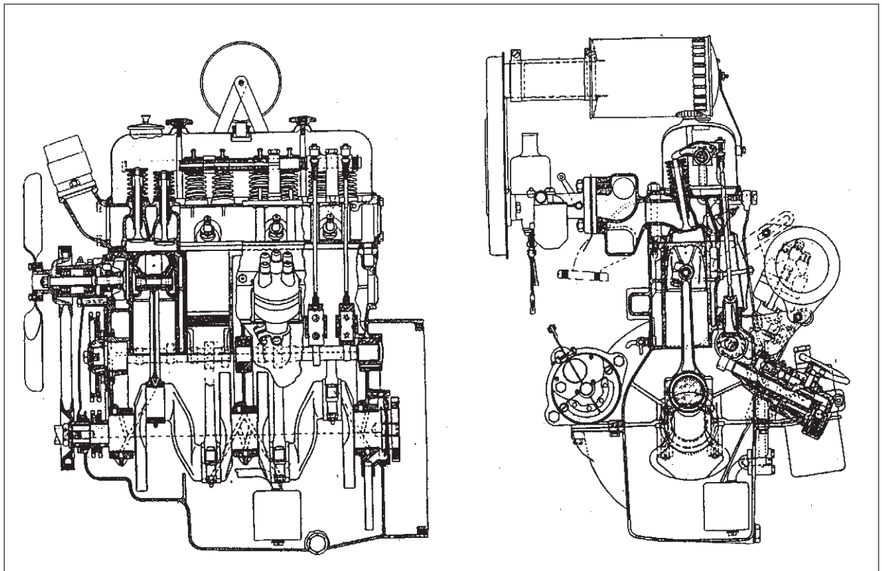
Cross and longitudinal sections of Morris Ten engine.
