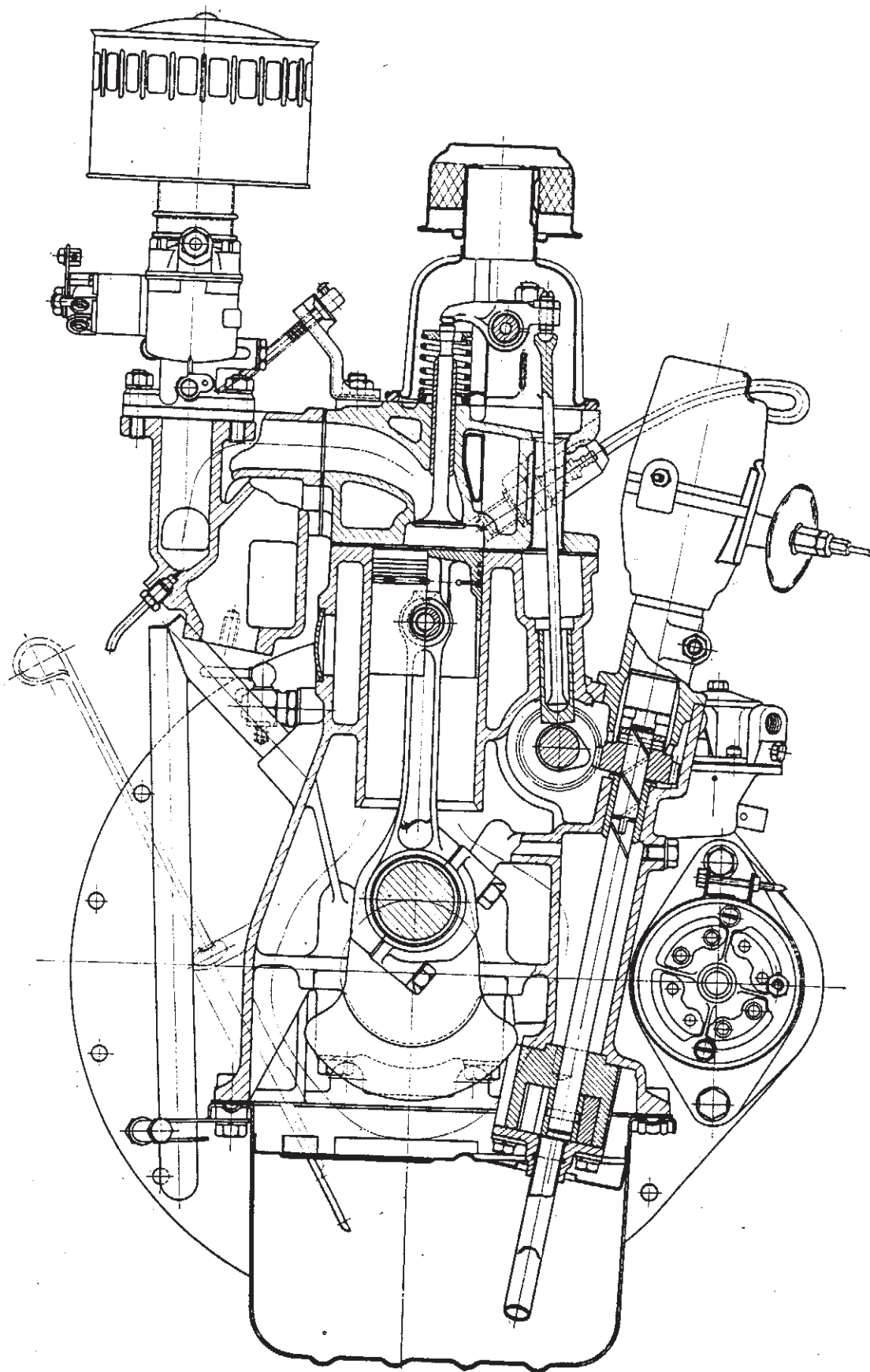
The original 803cc Standard Eight engine of 1953, that grew into that fitted to the MG Midget 1500 in 1974.
