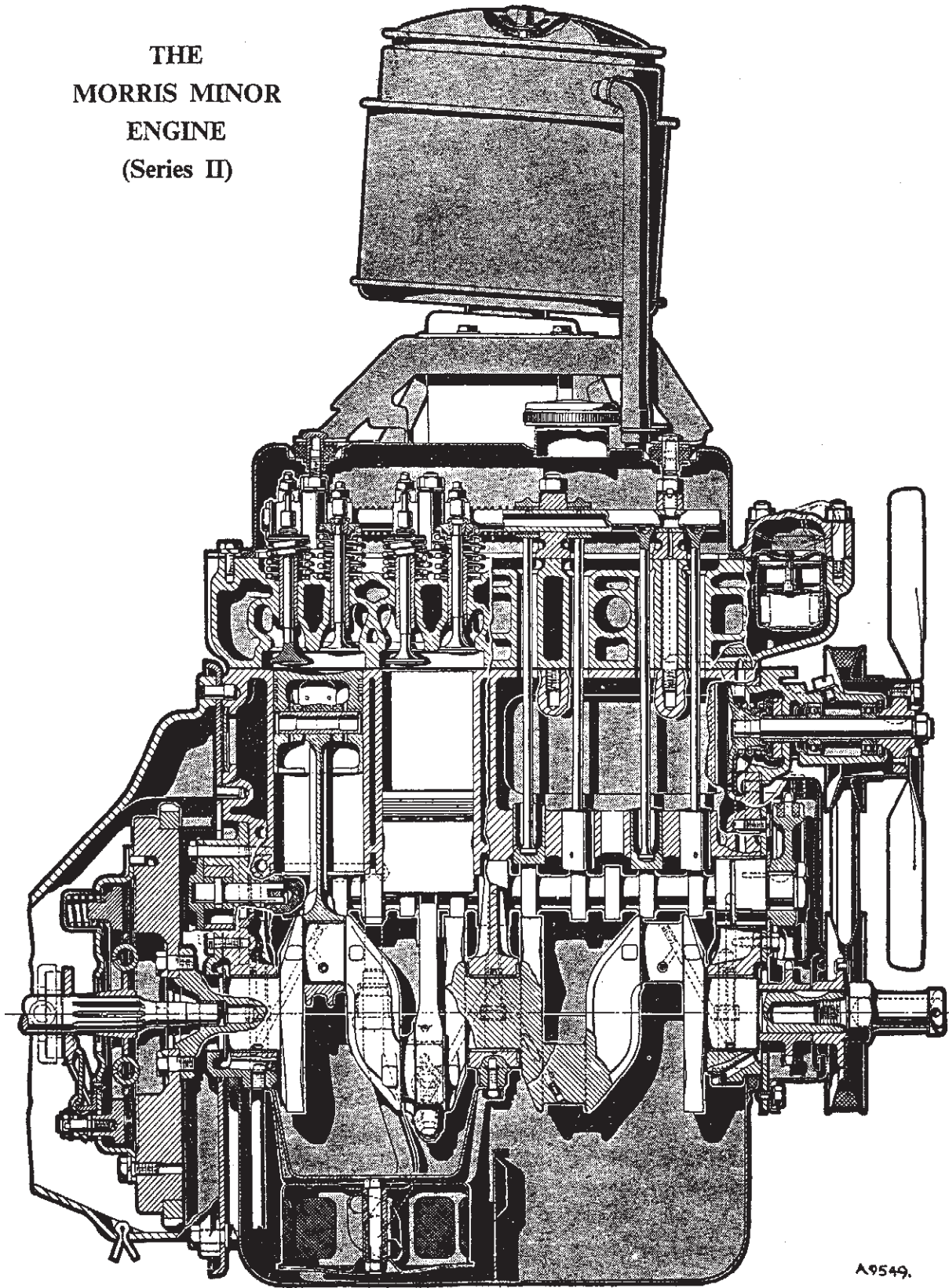
The Morris Minor 803cc 'A' series of 1954, enlarged to 948cc in 1956.
