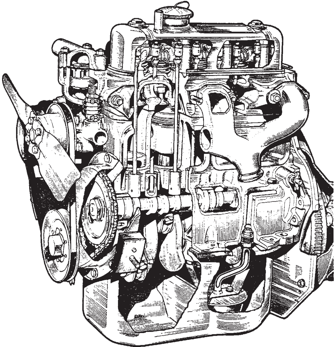
Cutaway view of the basic engine.
