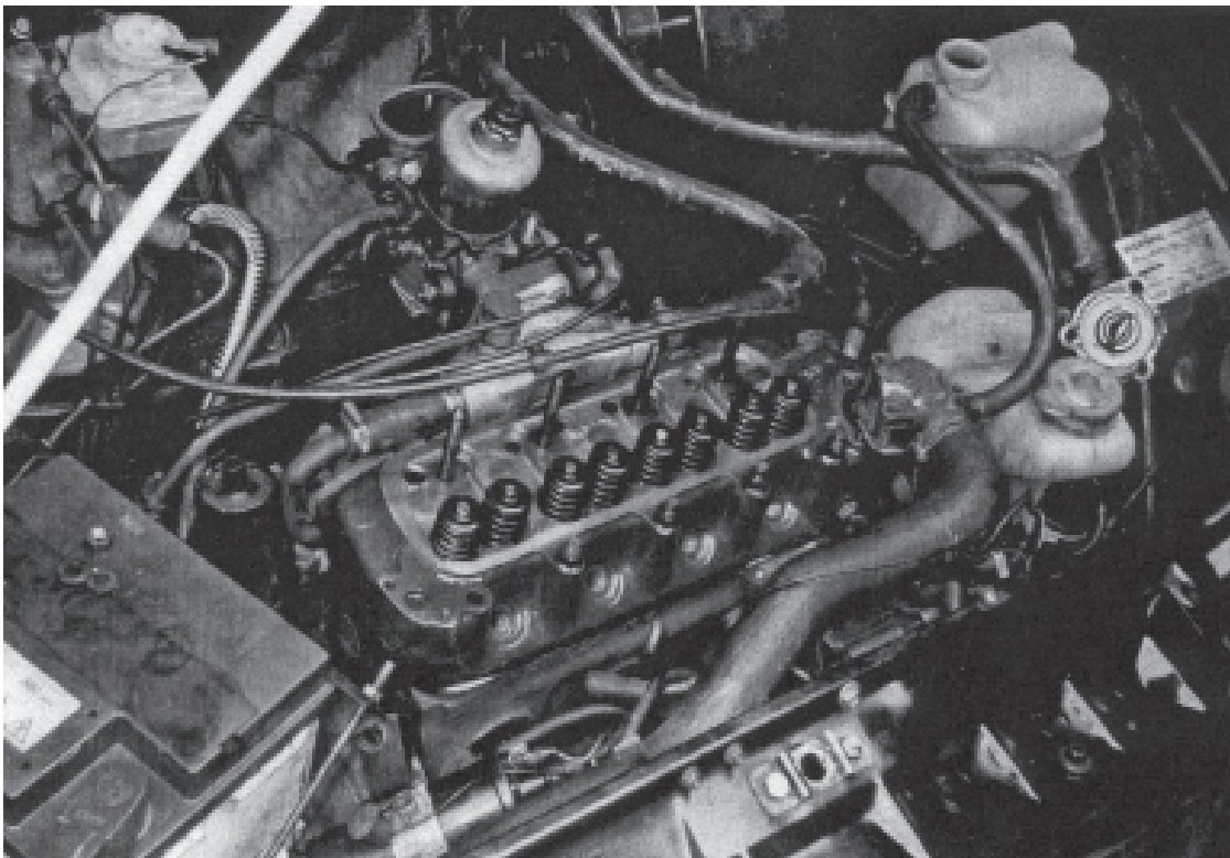
A 1300 MG Metro has its cylinder head swapped for a lead-free converted one.
