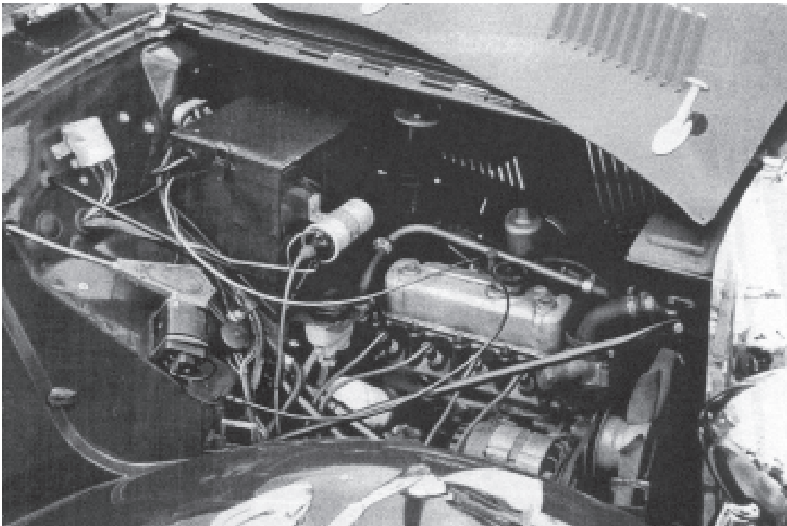
A MG YB saloon using a Morris Marina 1275cc 'A' series!
