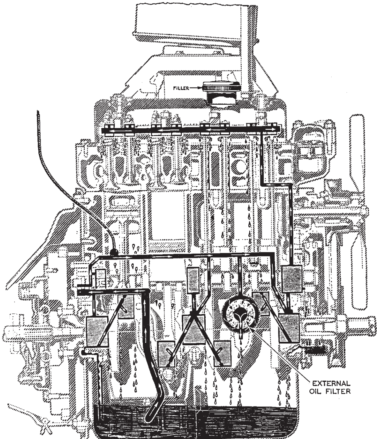
The early by-pass oil filter system of the 803cc 'A' Series, improved on the 948cc MG.
