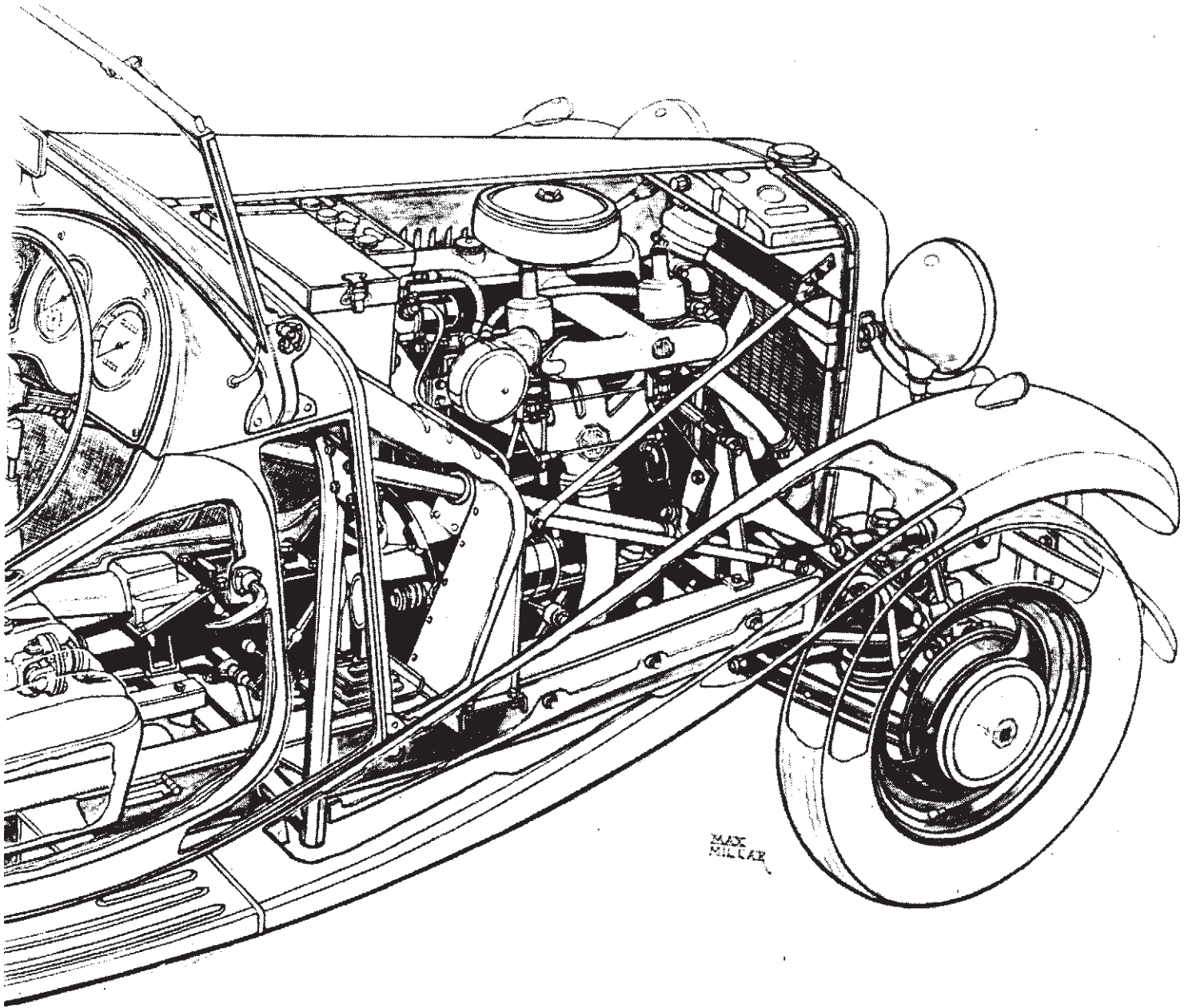
January 1950 saw the XPAG 1250cc engine fitted to the TD Midget. The unit was virtually unchanged from that fitted to the TC and was a twin carburetter version of the 1 1/4 litre saloon. Just look at all lovely access space with old type winged bonnets. Drawing copyright is that of Autocar magazine.
