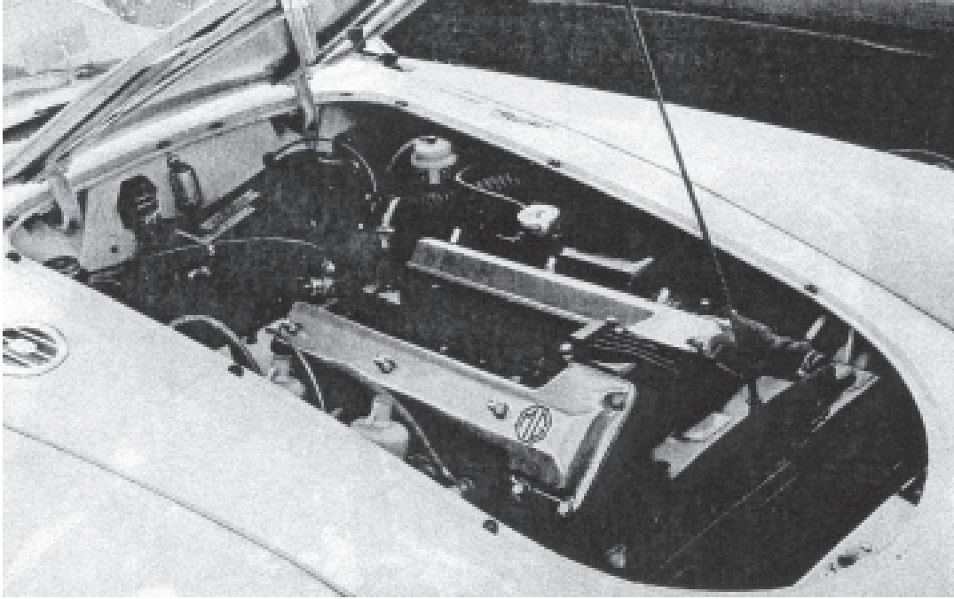
The MGA Twin Camshaft engine, snug in its bay.
