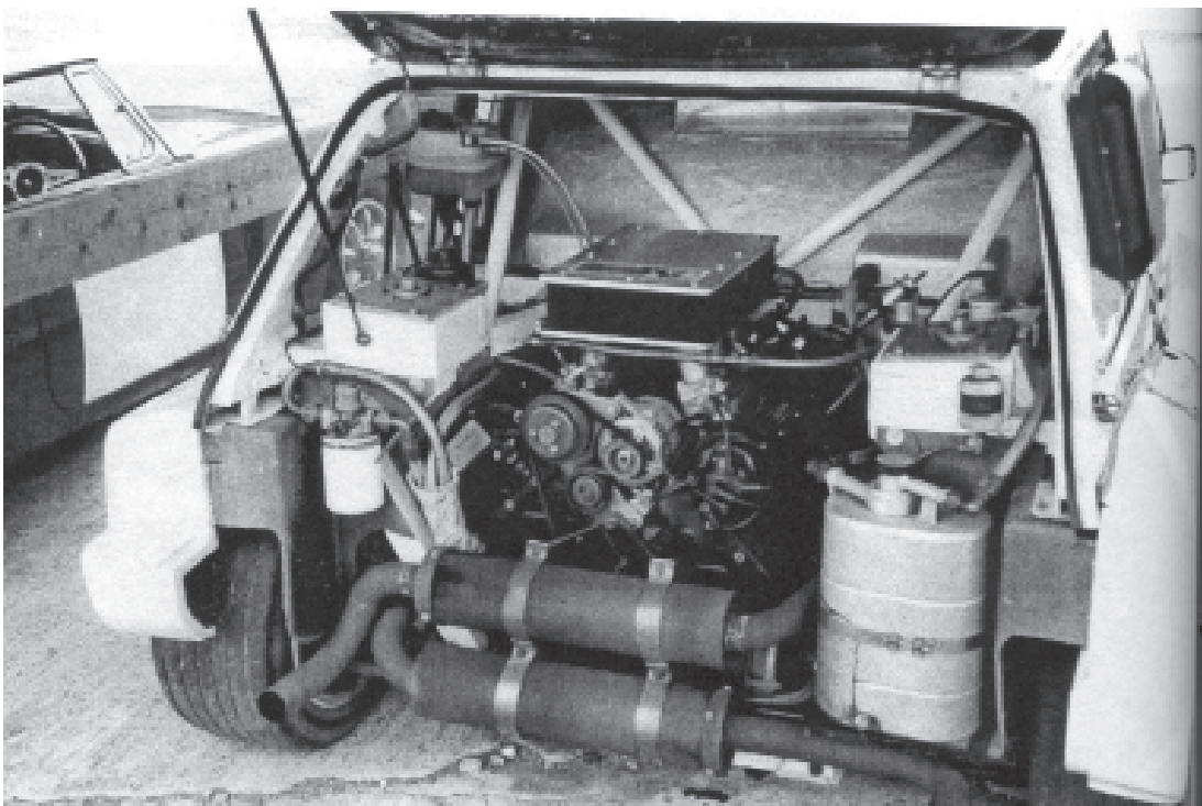
MG Metro 6R4, 'V64V' engine. A somewhat faster Metro!
