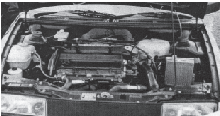
20 HE Rover M16 in a MG Montego
