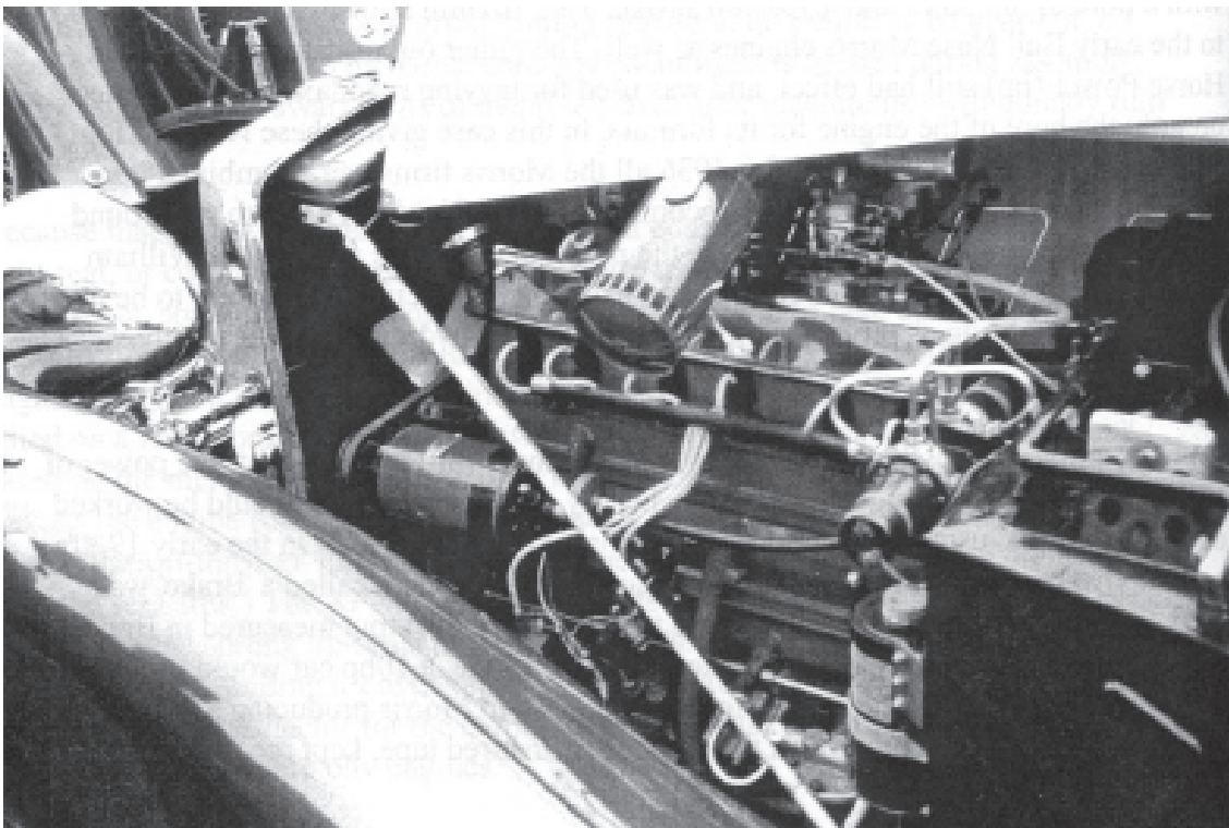
The related MG WA six cylinder overhead valve engine, showing tlc.
