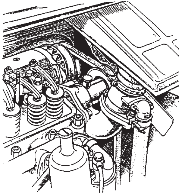
M.G. The overhead valves are operated by push rods on the T-type "Midget". Note the water pump and thermostat.
