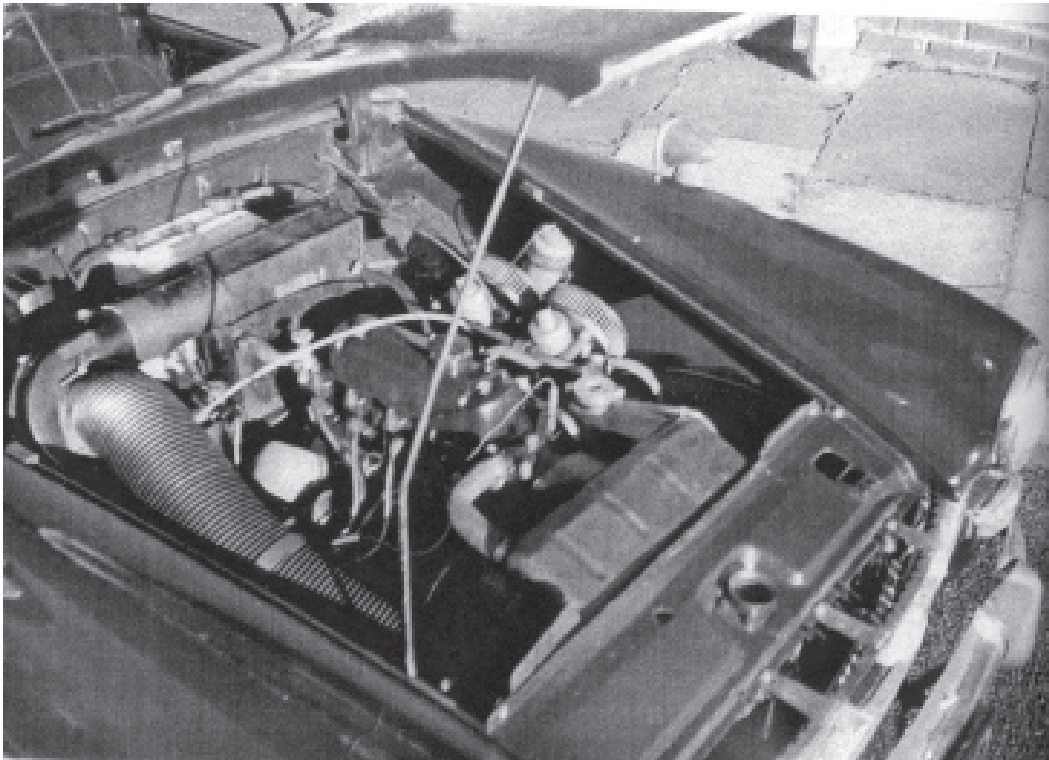
The Midget above has a Morris Marina 'A Plus' 1300 engine fitted, note the oil filter above the distributor.
