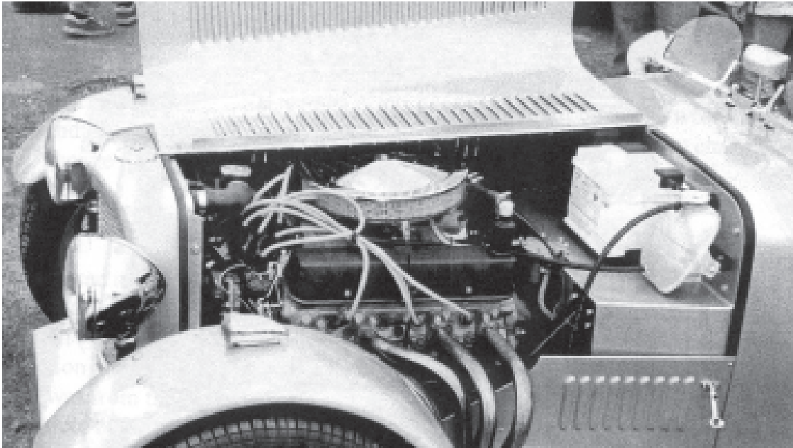
A V8 in a kit car based on MGB running gear.
