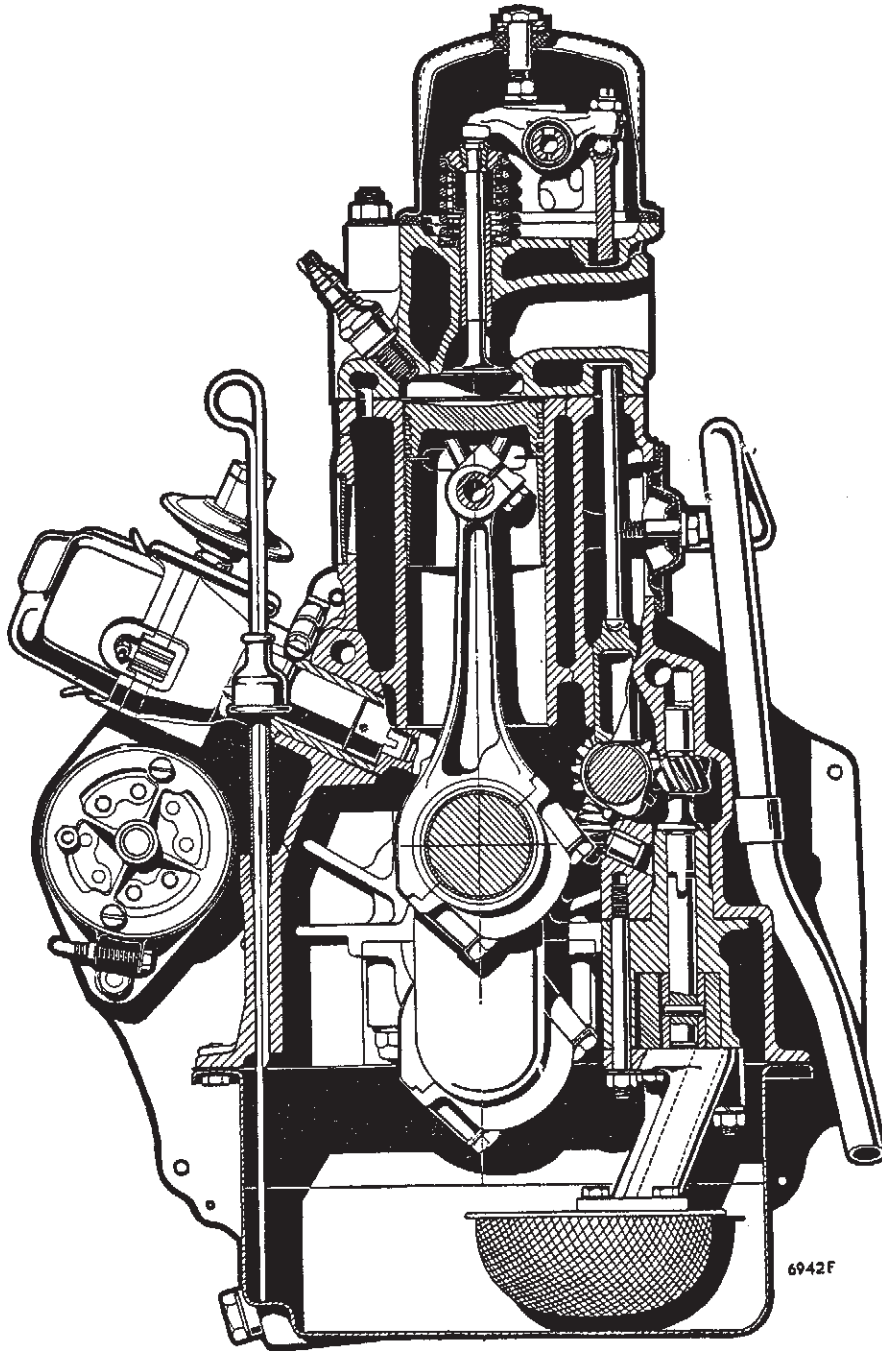
End view of a 1489cc 'B' series with later swan-neck breather pipe.
