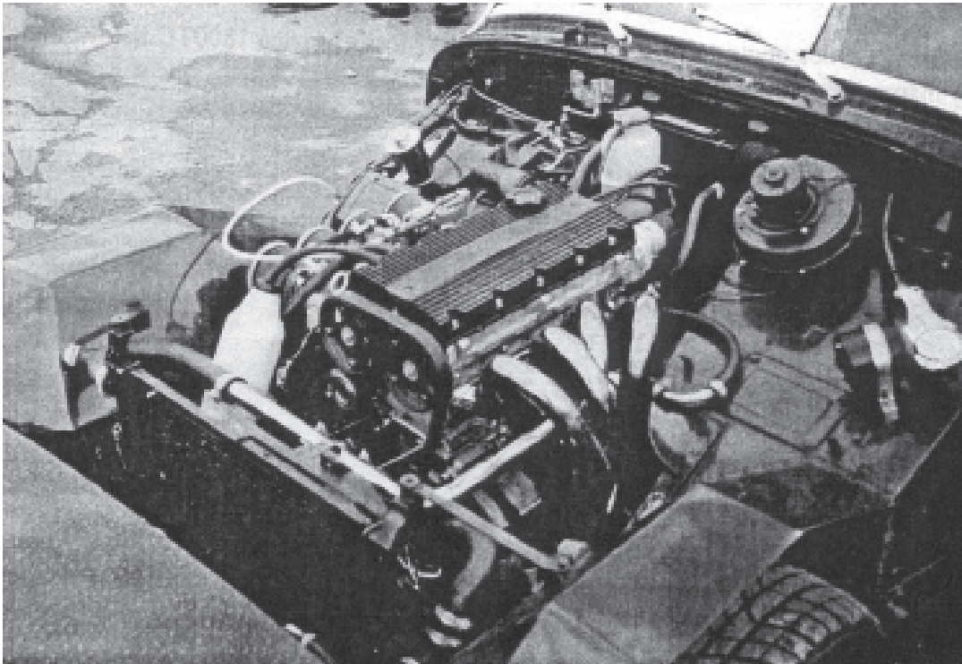
A Rover K16 engine in a special MG Midget.
