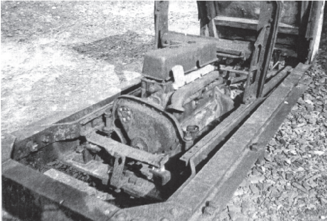
Industrial use of the sidevalve Morris 18hp six. Note the fume-extractor that looks like a rocker cover. Abandoned in a Welsh slate mine.
