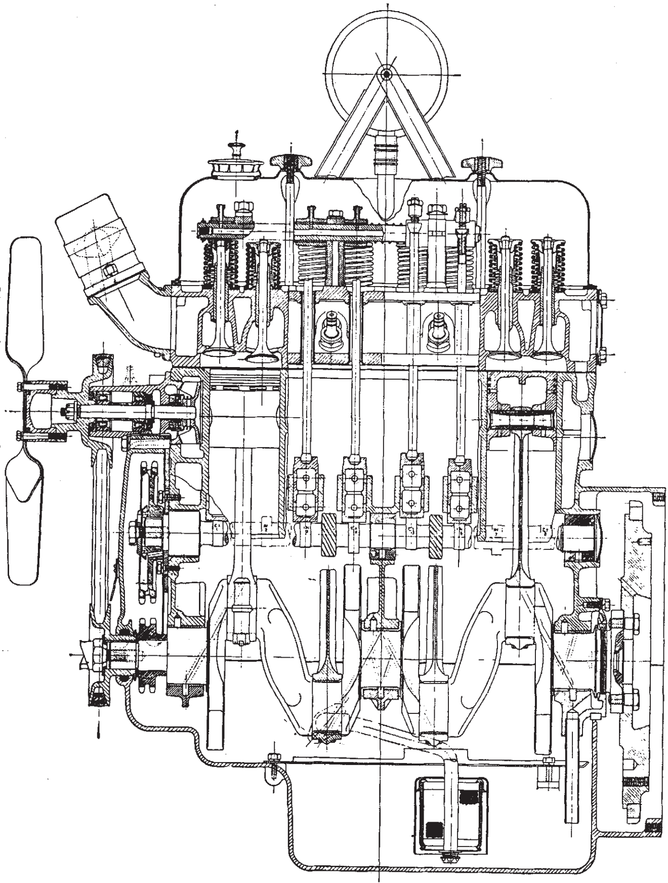
Side view of the 125cc carburettor XPAG/SC MG engine as fitted to the 'Y' series saloon in 1947, with the early smooth 9 pint sump.
