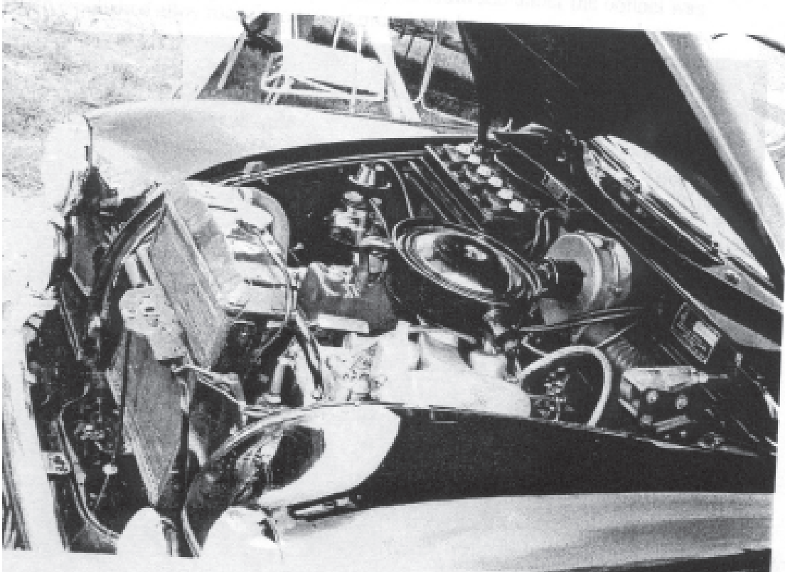
MG ZA underbonnet area. The 1489cc engine sits well forward.
