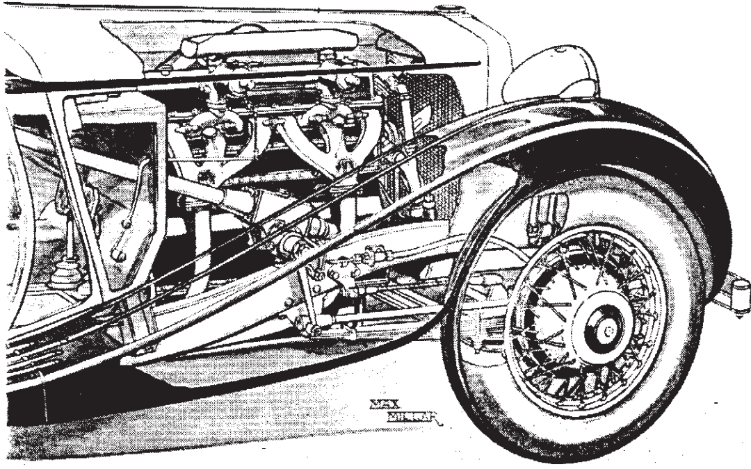
Down draught SU carburettors of the MG SA Two litre saloon, similar to those above.
