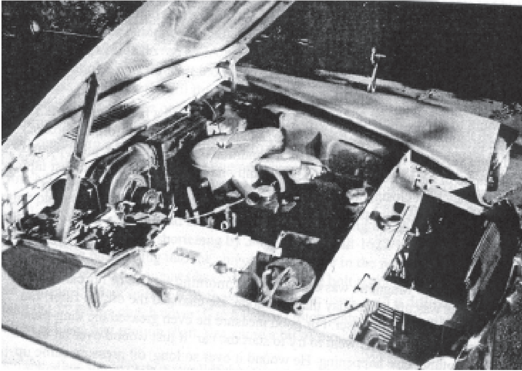
The 1622cc engine fitted to a Mk4 MG Midget, a close copy of the 1622cc MGA 1600 Mk2.
