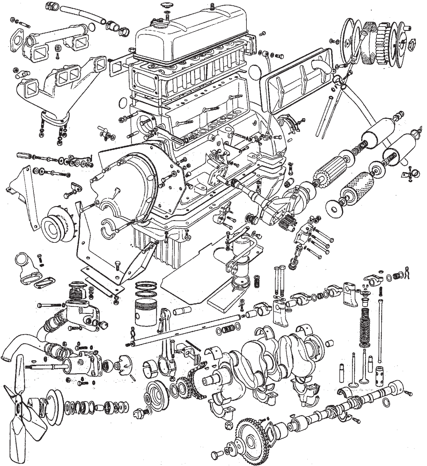
Components of the engine, showing cylinder block with push-rod cover and breather, cylinder head, sump, torque reaction link, oil pump, pick-up and alternative oil filters, manifolds (note inlet balance pipe), air cleaner, water pump parts, thermostat housing and bypass circuit, crankshaft and timing drive, connecting rod and piston assembly and valve train.
