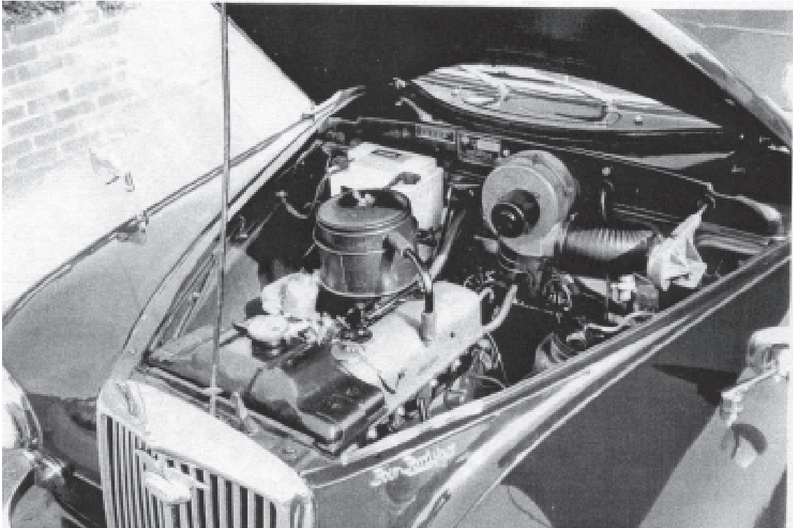
That fitted to the Wolseley 4/44, of 1952, was virtually the SC/2 engine of the MG YB.
