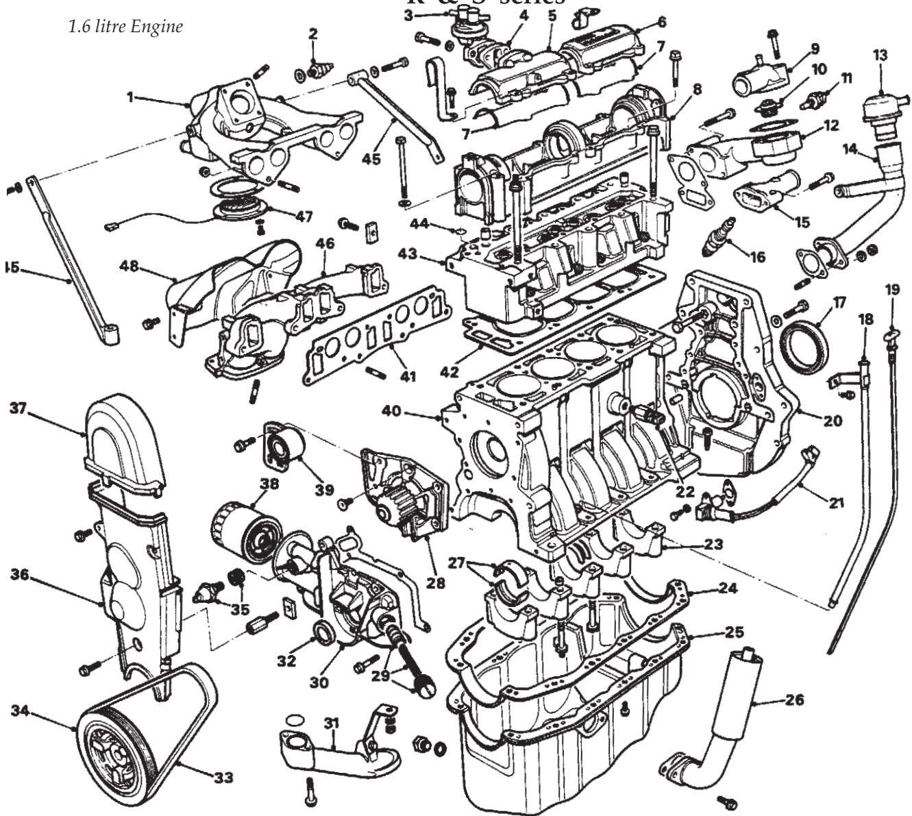
Exploded view of the 1.6 litre engine main components
