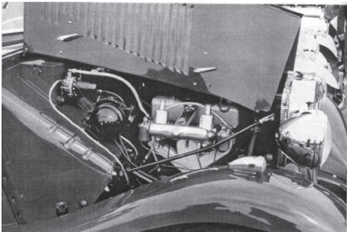
Very similar to look at, but this 1250cc XPAG MG TD engine is much more modern internally. Its Morris relation is the Morris Ten, series 'M'.
