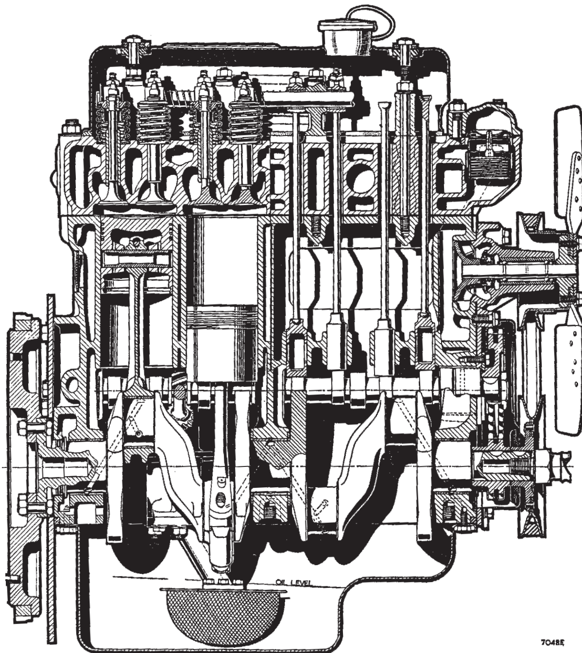
Side view of 1489cc 'B' series, with very early evacuated-below type the rthermostat.
